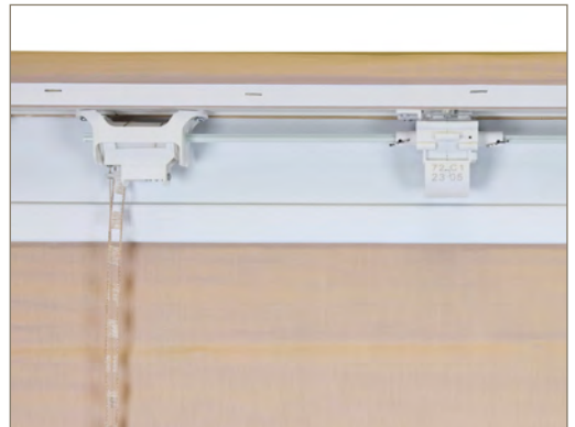
Cordless Spring and Spool
